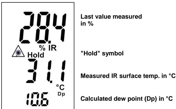
Figure 2-1: main menu/measuring mode
