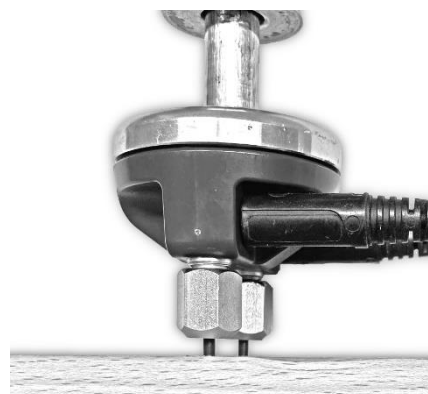
Figure 9-2: Use of Teflon-insulated pins
