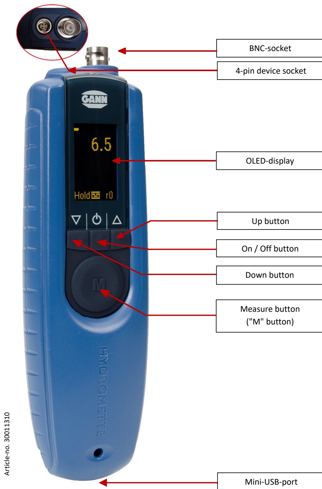
Figure 5-1: Front view of the Hydromette BL E 2
