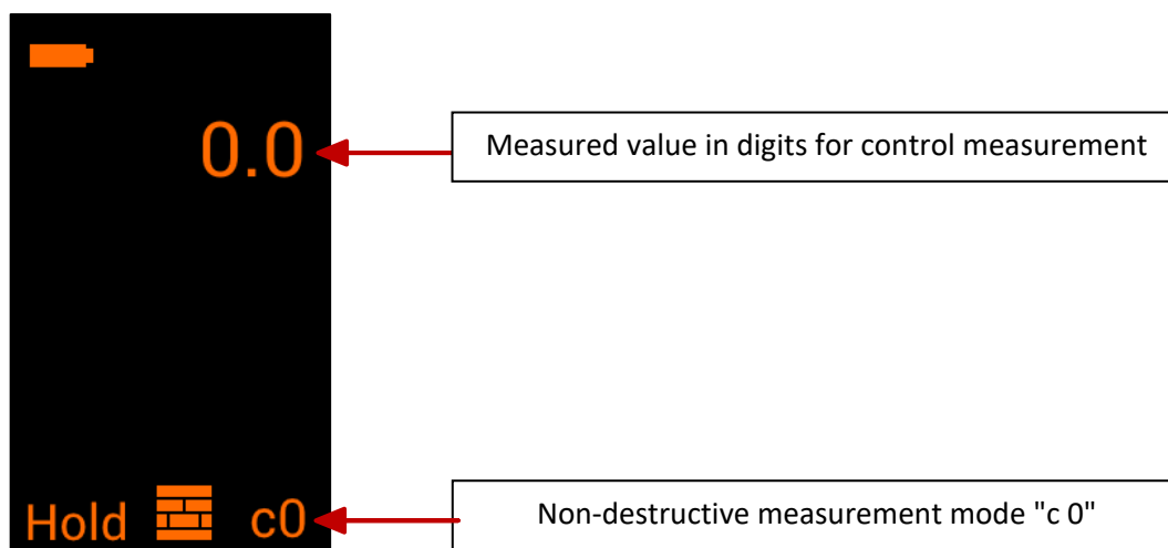
Figure 13-4: Capacitive measuring mode "c 0" display
